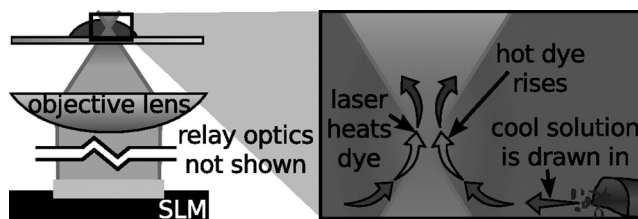
Figure 3. A spatial light modulator (SLM) is used to create multiple, controllable laser focused spots in the sample. These focused laser spots heat the dye solution, causing convection currents that create a flow towards the laser spots on the surface of the slide.
